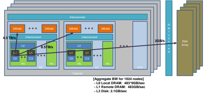
Fig. 3: An example system with 6 potential levels of CDs. Based on the configuration of [6].
