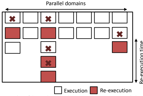
Fig. 7: Example of 7 nodes, each executing 2 sequential child CDs. Some CDs fail and require re-execution, which is overlapped between nodes with uncoordinated recovery.
