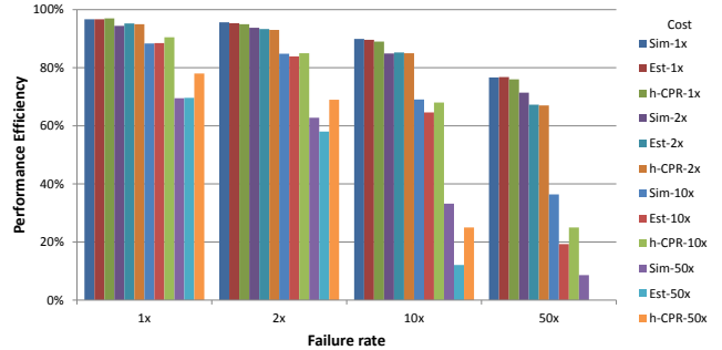
Fig. 8: Comparison of the CD simulator and an h-CPR analytical model [37]
