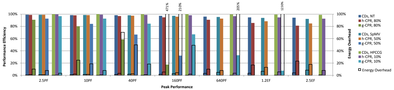
Fig. 9: Performance efficiency (solid bars) and energy overheads (clear bars) with CDs, h-CPR, and g-CPR for the three applications across a range of system scales. For each application, we indicate the equivalent fraction of memory preserved by the checkpointing schemes. Note that g-CPR fails to complete execution with some applications and scales and often incurs very high energy overheads.
