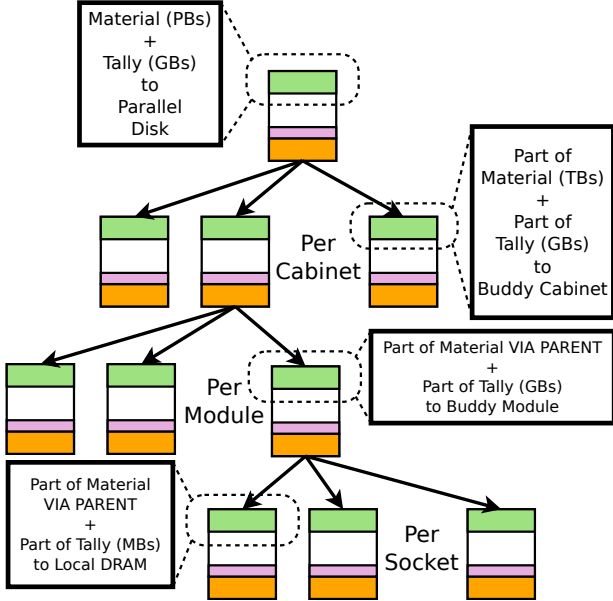
Fig. 4: Mapping example of neutron transport.
